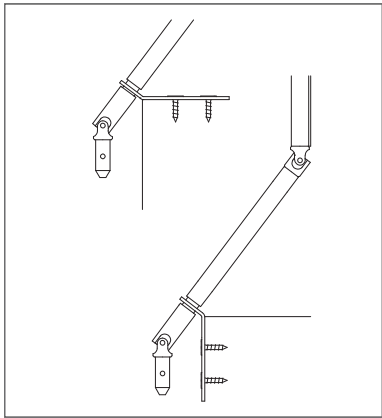
Pivot bearing for gear and crank rods
