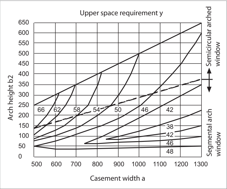
D dimension and top space requirement for round and segmental arch windows
